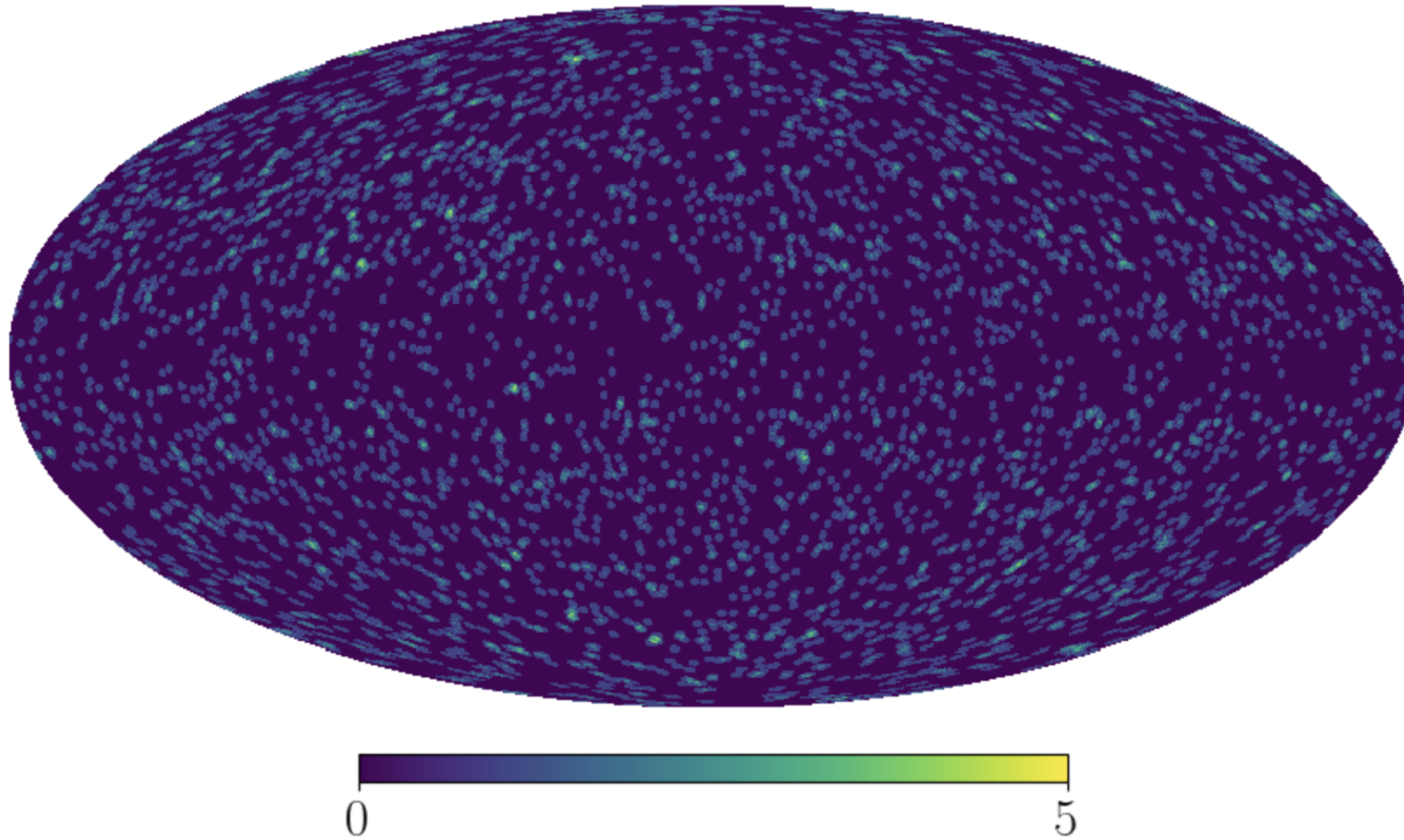
Mollweide view
