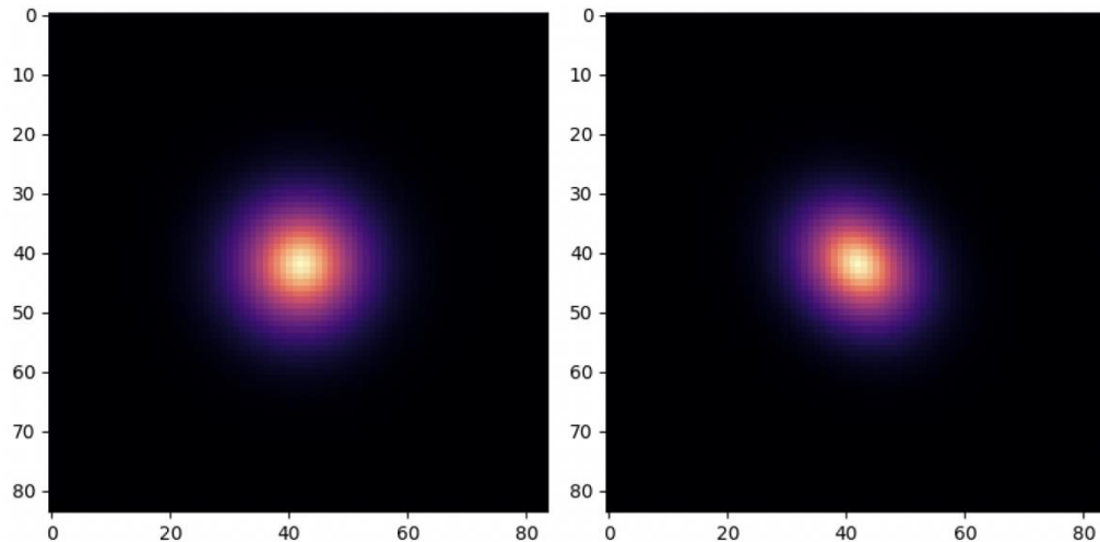
(e) \kappa
