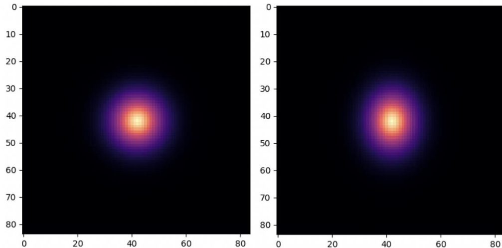
(a) Unlensed
